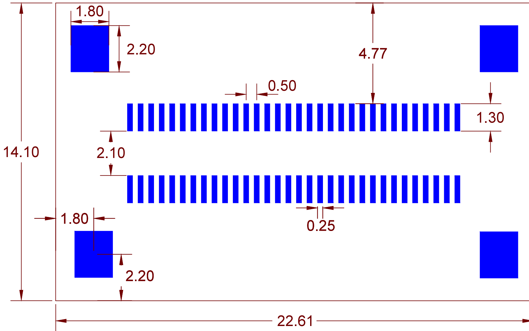
SOLDER MASK
